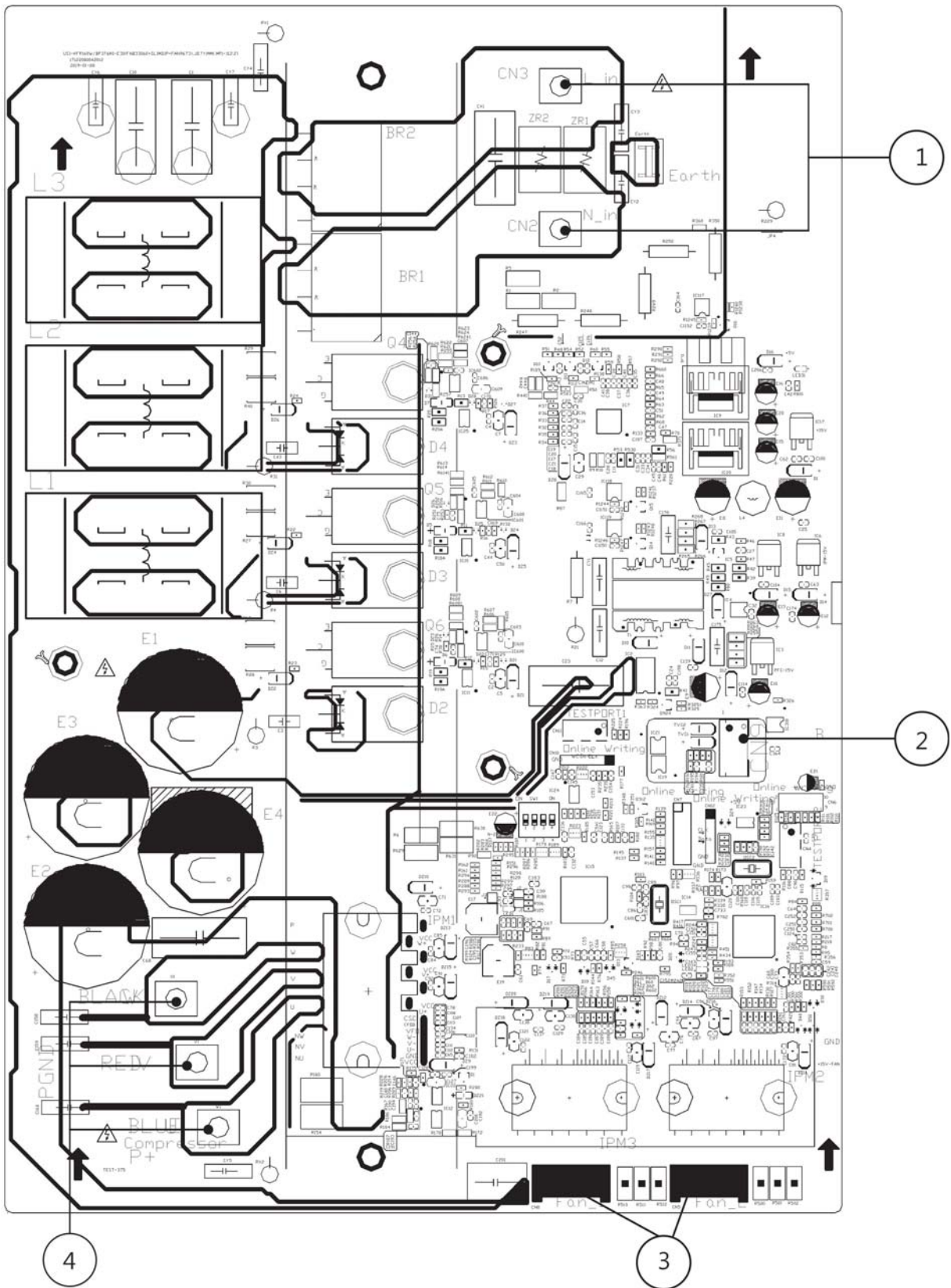
Outdoor unit IPM board diagram: 1712200042012
